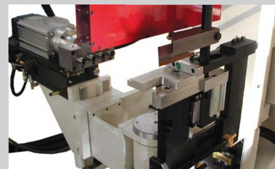
FLEX-45 Sawing and drilling station at 90°
