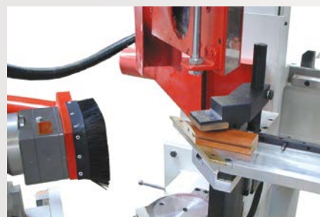
FLEX-45 Sawing and drilling station at 45°
